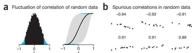
Figure 2 | Correlation coefficients fluctuate in random data, and spurious correlations can arise. (a) Distribution (left) and 95% confidence intervals (right) of correlation coefficients of 10,000 n = 10 samples of two independent normally distributed variables. Statistically significant coefficients ( \alpha = 0.05 ) and corresponding intervals that do not include r = 0 are highlighted in blue. (b) Samples with the three largest and smallest correlation coefficients (statistically significant) from a.
